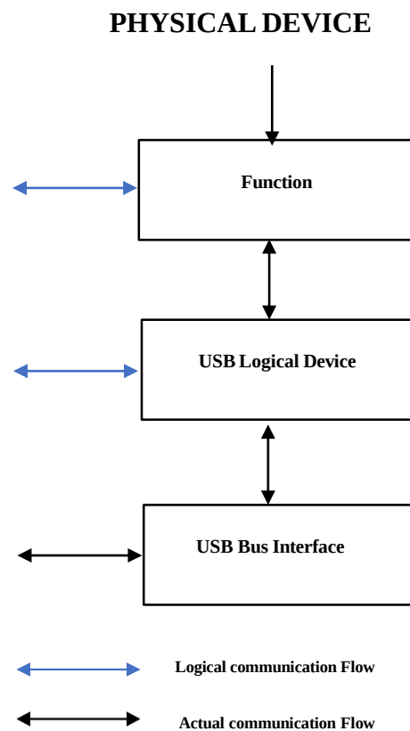
Fig No 4.1 Physical Device Composition
